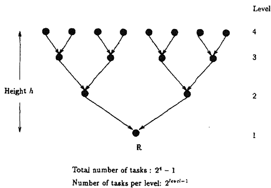
Fig. 1. Example of a complete binary intree with height = 4.
