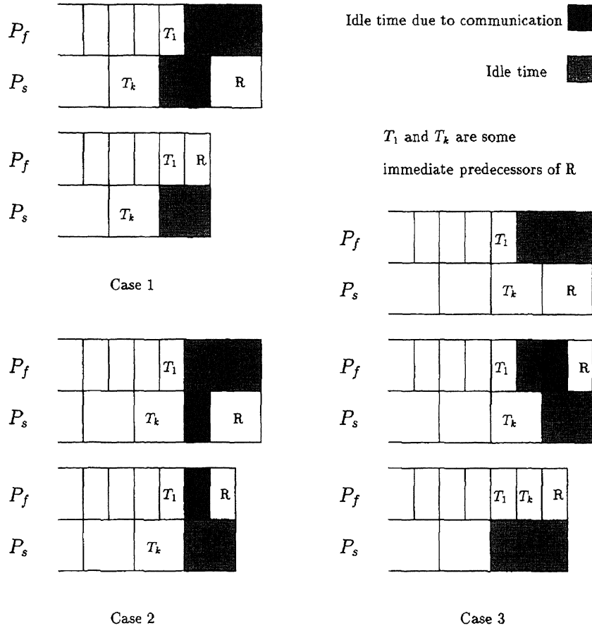
Fig. 2. Allocation of the root for the optimality.
