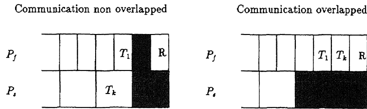
Communications can be overlapped without increasing the schedule length
